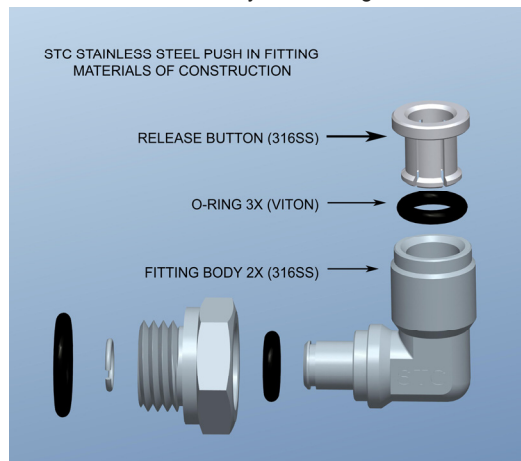
Collet Style SS Fitting
