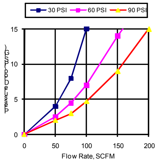
AF4000 Series Filter Flow Rate VS Pressure Drop @ 30, 60, 90 PSI Supply Pressure
